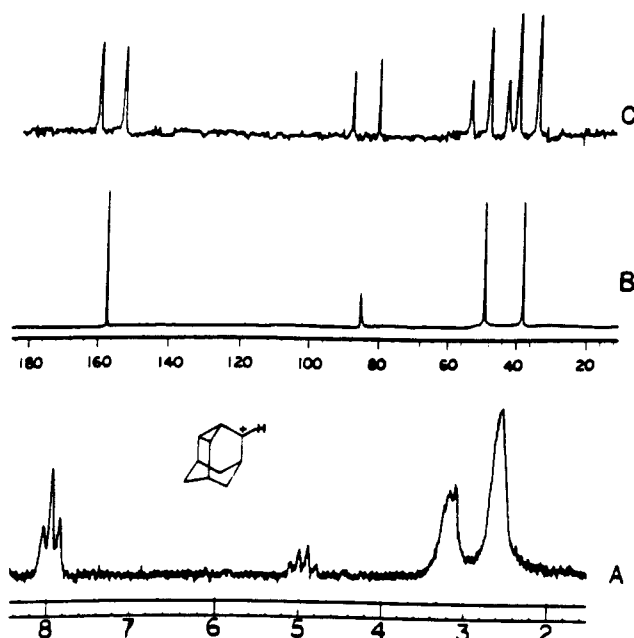
Figure 3. NMR spectra for 8,9-dehydro-2-adamantyl cation (40 or 41): (A) ^1\text{H} NMR (60 MHz) spectrum of in \text{FSO}_3\text{H-SO}_2\text{-ClF} at -120^\circ\text{C} ; (B) proton-decoupled ^{13}\text{C} NMR spectrum; (C) proton-coupled ^{13}\text{C} NMR spectrum (reprinted from ref 34; copyright 1978 American Chemical Society).
